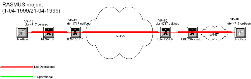
[fig 6] Initial network topology
